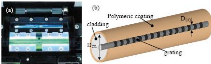
(a) Quartz moulds of the recoater machine (b) Schematic diagram of the uniformly coated FBG.
